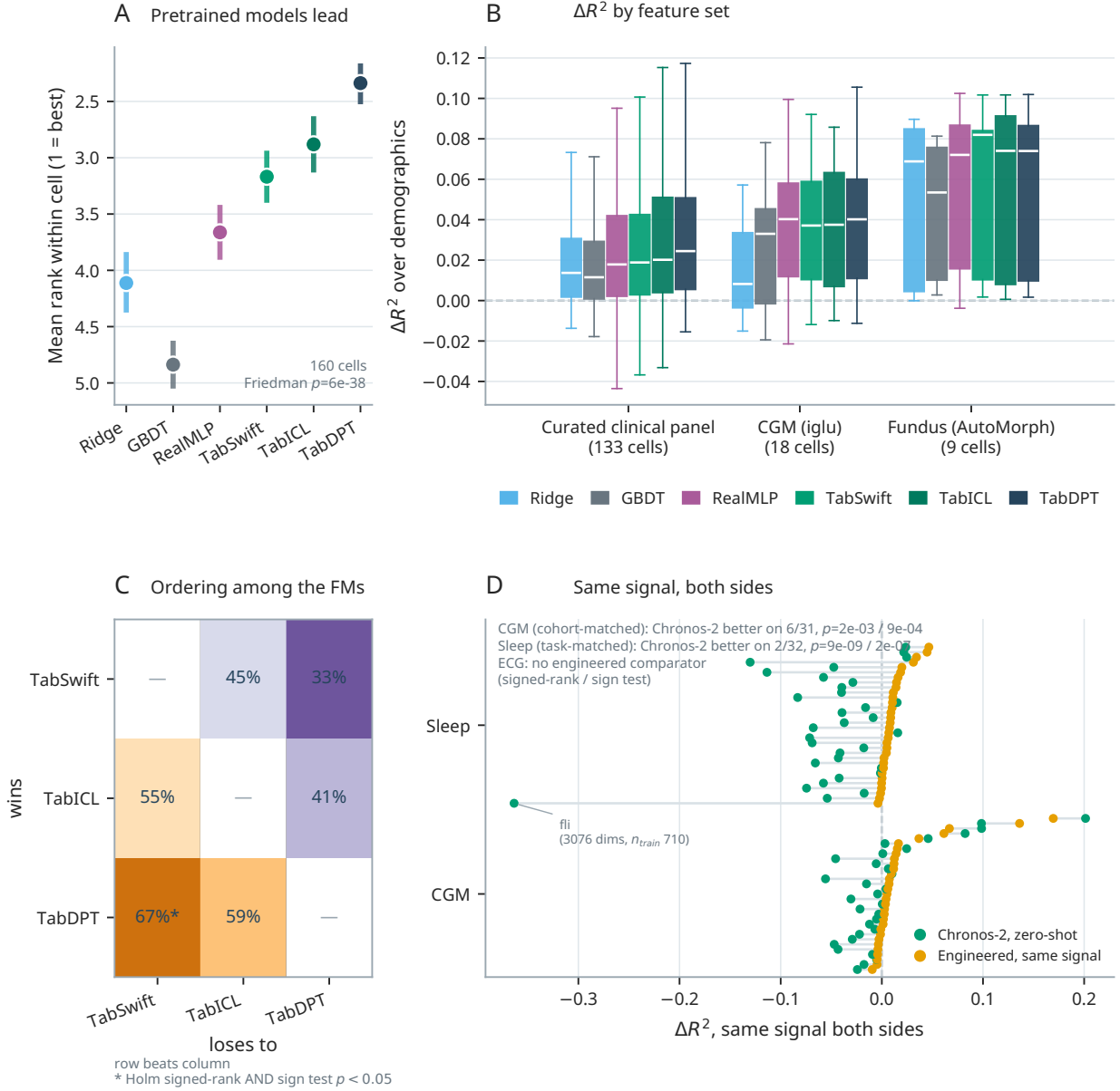
Figure 3 | Model families on matched clinical comparisons. A , Mean rank of each method within a comparison cell (1 = best) across 160 cells in which all six methods ran on the same task, cohort, feature set, and split, spanning 52 tasks; bars are bootstrap 95% intervals. B , \Delta R^2 over demographics by feature set; boxes show quartiles, whiskers 1.5 IQR, outliers omitted; cell counts differ and the fundus and glucose groups are thin. C , Fraction of cells in which the row model exceeded the column model among the pretrained tabular models; the asterisk marks the one pair significant after Holm correction under both a signed-rank and a sign test. D , Frozen zero-shot Chronos-2 embeddings are compared with engineered features from the same signal using the same ridge head. CGM pairs share tasks and cohorts; WatchPAT pairs are matched on task only and use different cohorts. The labeled fatty-liver-index failure combines a 3,076-dimensional embedding with 710 training participants; the demographics-only baseline reached R^2 = 0.79 . \Delta R^2 is measured against the same demographics-only ridge baseline within each cell.
