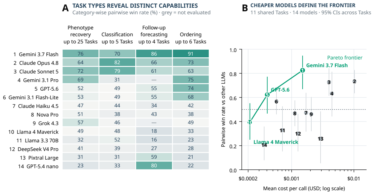
Figure 4 | Cohort data maps LLM capability and efficiency. A , Each cell is a model’s within-category pairwise win rate against other LLMs, computed only from available head-to-heads on the same task; values are percentages and higher is better. Rows are ordered by overall win rate on the 11 tasks shared by all 14 models. Grey cells indicate that a model was not evaluated in that category. Category coverage differs, and native metrics are never compared across categories. B , Pairwise win rate against other LLMs on the 11 shared tasks versus mean cost per call. Vertical lines are 95% bootstrap confidence intervals across tasks; numbers identify model rows in A. A model remains on the Pareto frontier when every cheaper model has a lower win rate.
