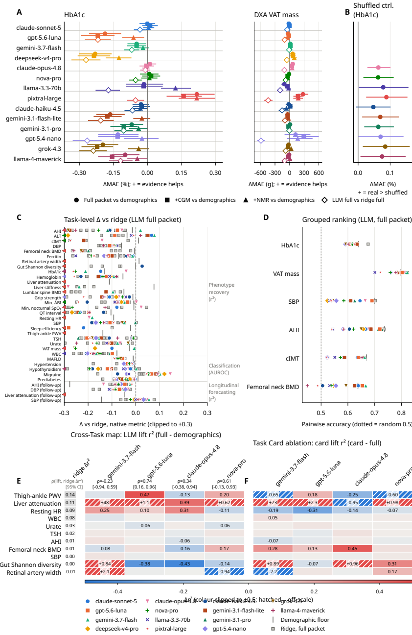
Supplementary Figure 4 | PhenoBench-LLM paired and mechanistic analyses. A , Paired MAE effects of evidence arms and the fitted probe for HbA1c and VAT mass. B , HbA1c shuffled-packet control. C , Per-Task full-packet difference from the fitted probe. D , Grouped-ranking pairwise accuracy with random, demographic-order and ridge-order references. E , Cross-Task map of full-packet R^2 lift over demographics, ordered by fitted-probe lift. F , sanitized Task Card R^2 shift over the full packet. Off-scale heatmap values are printed and hatched. All comparisons use the validation split and retain null and negative estimates.
