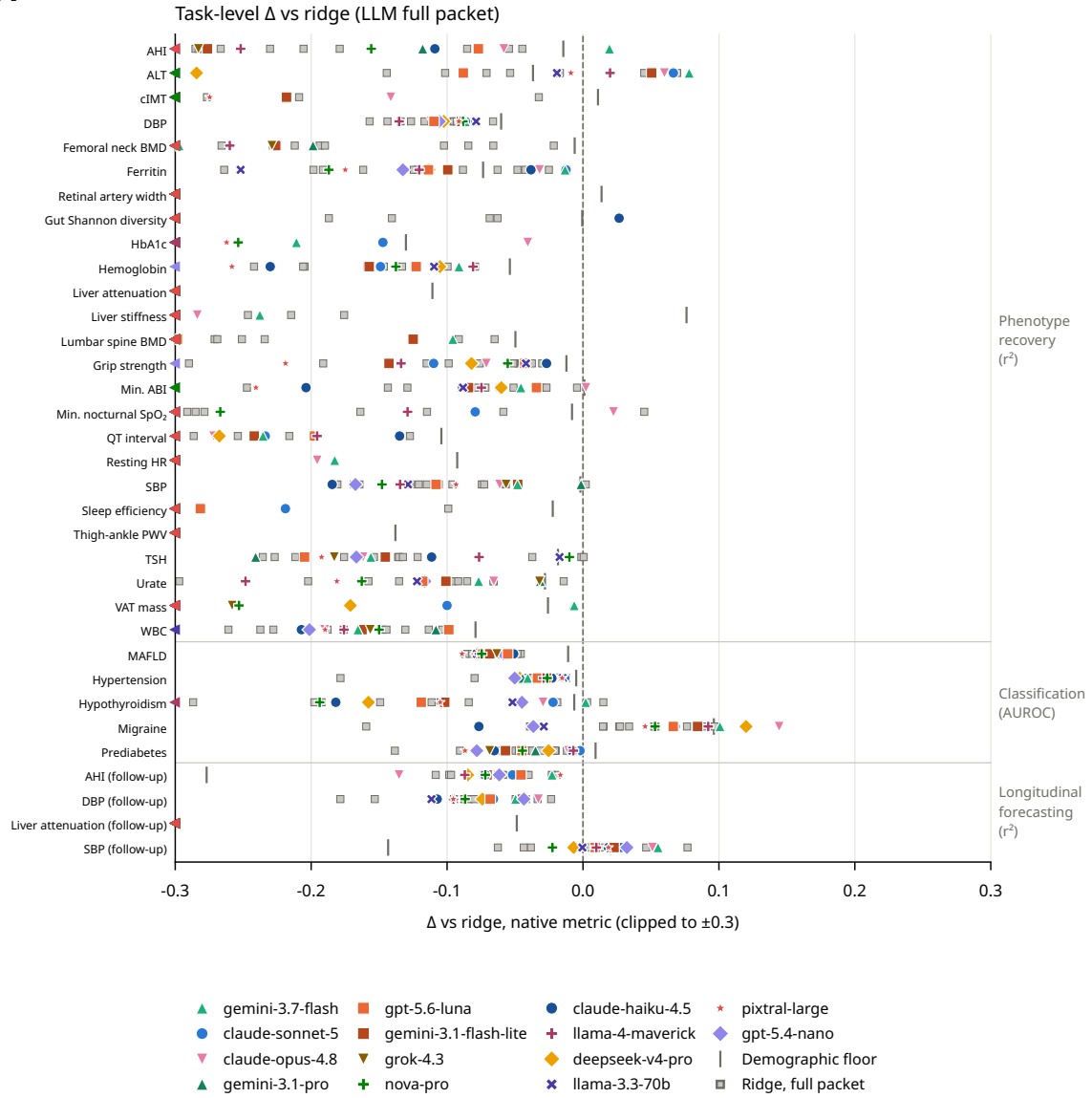
Supplementary Figure 5 | Task-level PhenoBench-LLM effects against fitted probes. Each marker is one model's full-packet primary-metric difference from the ridge or logistic probe over the same fields; zero denotes the fitted probe. Grey ticks show the demographic-floor difference from the probe and grey squares show the Task Card arm where available. Values outside \pm 0.3 are marked at the edge and retained exactly in the source table. Tasks are grouped by phenotype recovery, classification and longitudinal forecasting; grouped ranking is shown in Supplementary Figure 4.
